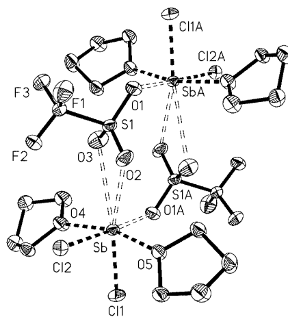
Figure 2. Molecular structure of 2 ·2THF in the solid state; selected distances (Å) and angles (°): \text{Sb–Cl1} 3.3628(8), \text{Sb–Cl2} 2.3629(8), \text{Sb–O1A} 2.876(3), \text{Sb–O2} 2.911(3), \text{Sb–O3} 3.084(3), \text{Cl1–Sb–Cl2} 92.75(3), \text{Cl1–Sb–O1A} 82.57(5), \text{Cl1–Sb–O2} 158.83(5), \text{Cl1–Sb–O3} 153.55(5).
