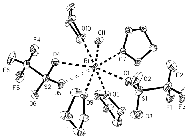
Figure 1. Molecular structure of 1 ·4THF in the solid state; selected distances (Å) and angles (°): \text{Bi–Cl1} 2.465(4), \text{Bi–O1} 2.386(11), \text{Bi–O4} 2.613(13), \text{Bi–O5} 2.879(15), \text{Cl1–Bi–O8} 156.4(3), \text{Cl1–Bi–O5} 131.2(3), \text{Cl1–Bi–O4} 80.4(3).
